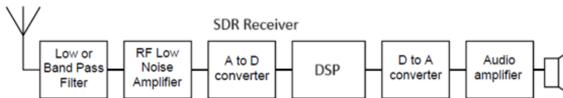
The direct sample SDR block diagram.
