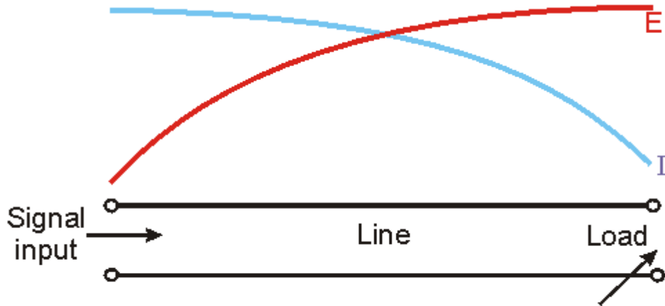
A line terminated with an open-circuit
