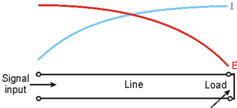
A line terminated with a short-circuit
